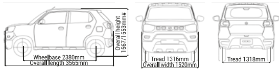
*Height = 1553 for Std and LXi variant. The drawings shown are general specifications of the vehicle.
